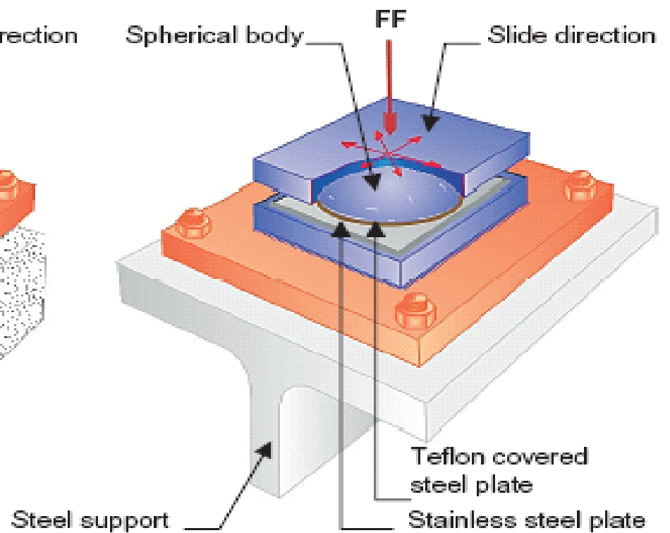
Slide bearing
