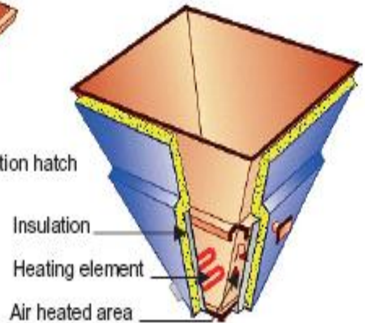
Bottom with heated area (Optional)
