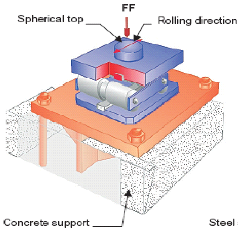
Roller bearing
