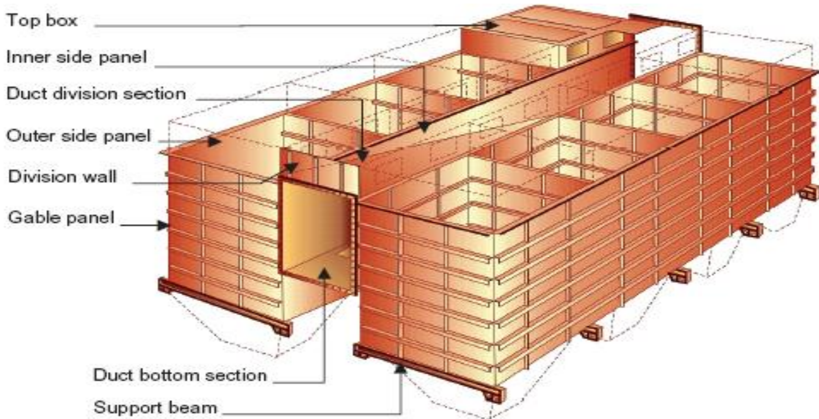
Casing single type
